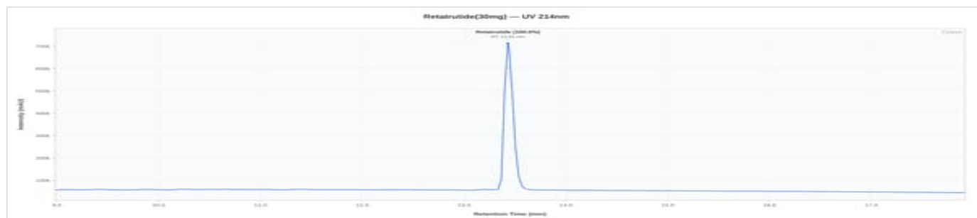
Retatrutide (RT30) 30mg - PPA-CP-RT30-C6001: UV Chromatogram
